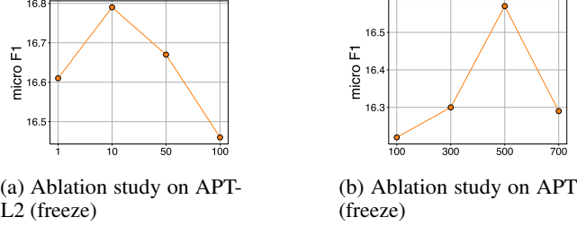
Figure 10: Performance of our model on dd242 w.r.t varying \{\lambda_j\} .
