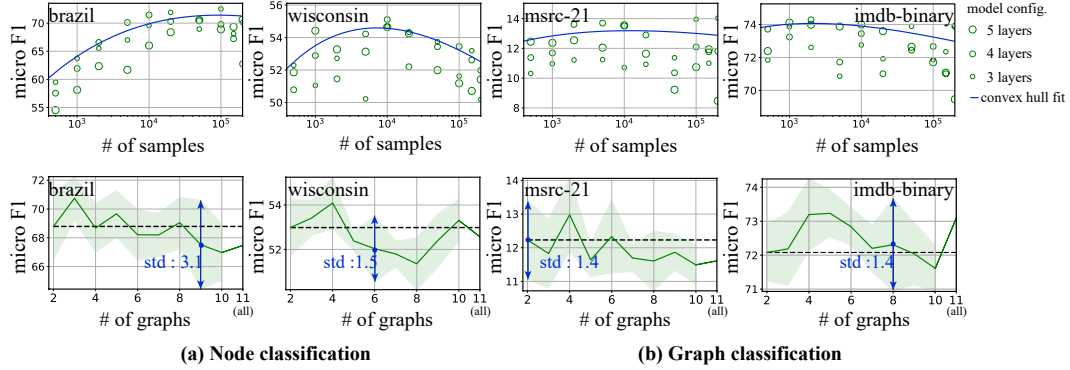
Figure 1: Top row : The effect of scaling up sample size (log scale) on the downstream performance based on a group of GCCs [52] under different configurations (the graphs used for pre-training are kept as all eleven pre-training data in Table 3, and the samples are taken from the backbone pre-training model according to its sampling strategy). The results for different downstream graphs (and tasks) are presented in separate figures. To better show the changing trend, we fit a curve to the best performing models ( i.e. , the convex hull fit as [1] does). Bottom row : The effect of scaling up the number of graph datasets on the downstream performance based on GCC. For a fixed horizontal coordinate, we run 5 trials. For each trial, we randomly choose a combination of input graphs. The shaded area indicates the standard deviation over the 5 trials. See Appendix E for more observations on other graph pre-training models and detailed settings.
